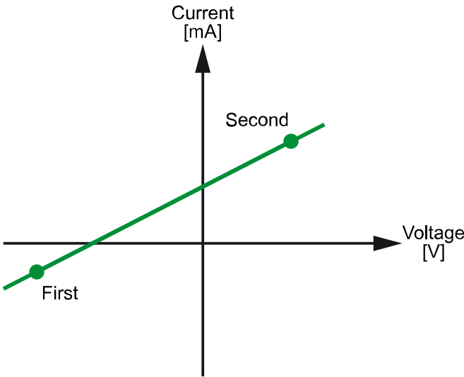
Figure 35. Analog input current set value scaling – Set value
