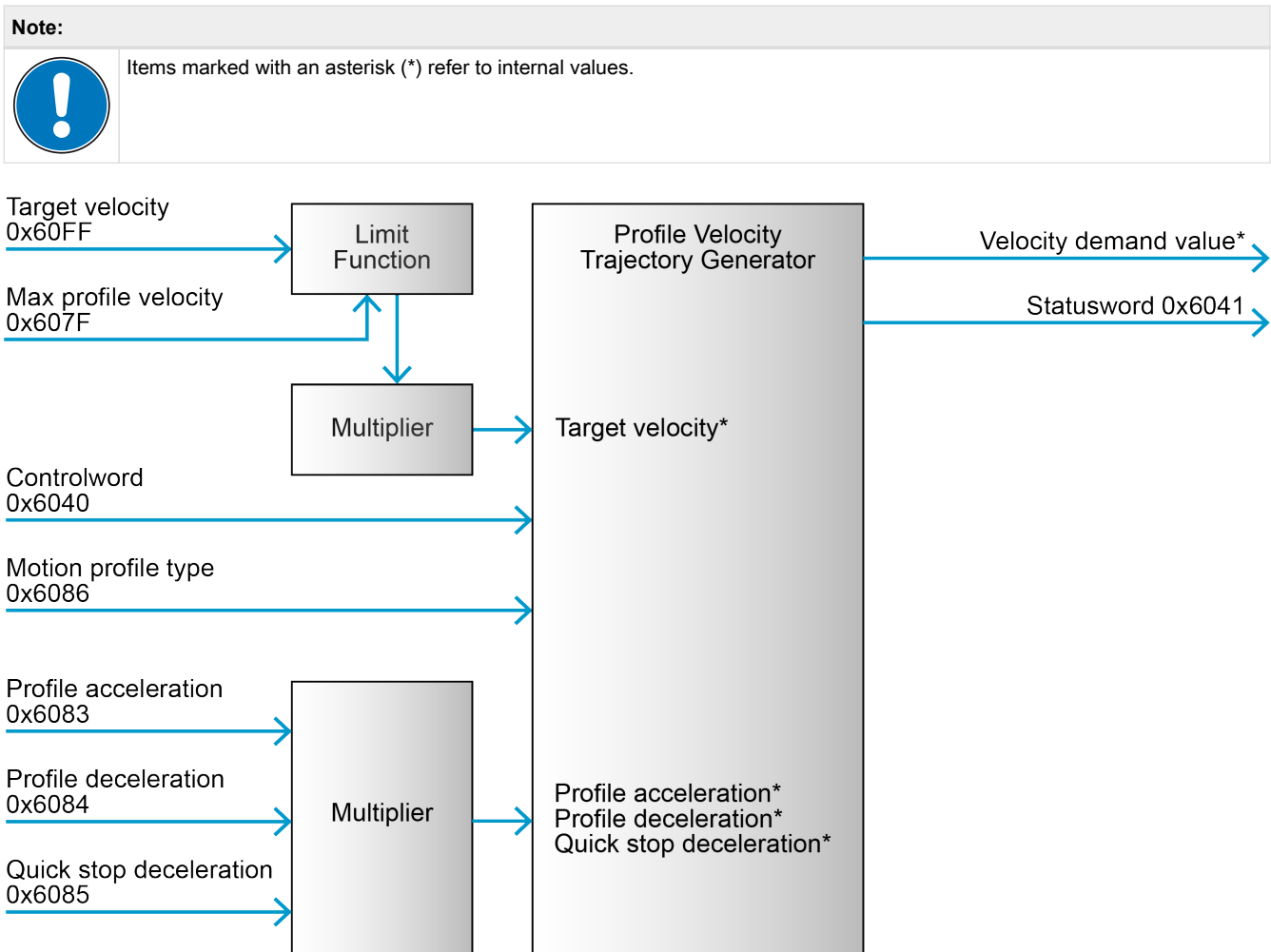
Figure 5. Profile Velocity Mode - block diagram
