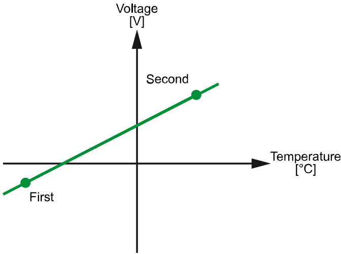
Figure 40. Analog output temperature monitor scaling
