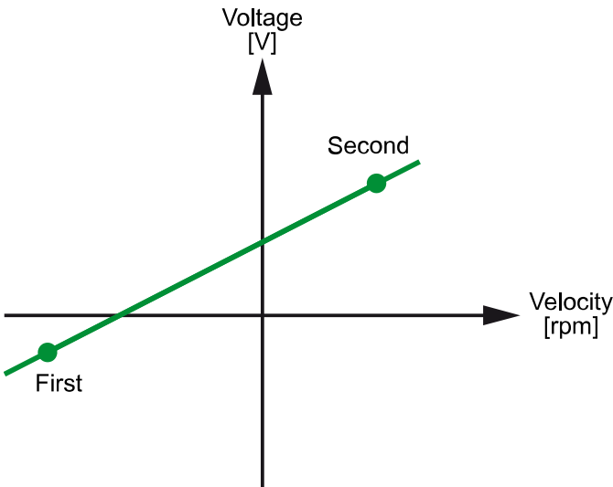
Figure 38. Analog output velocity monitor scaling
