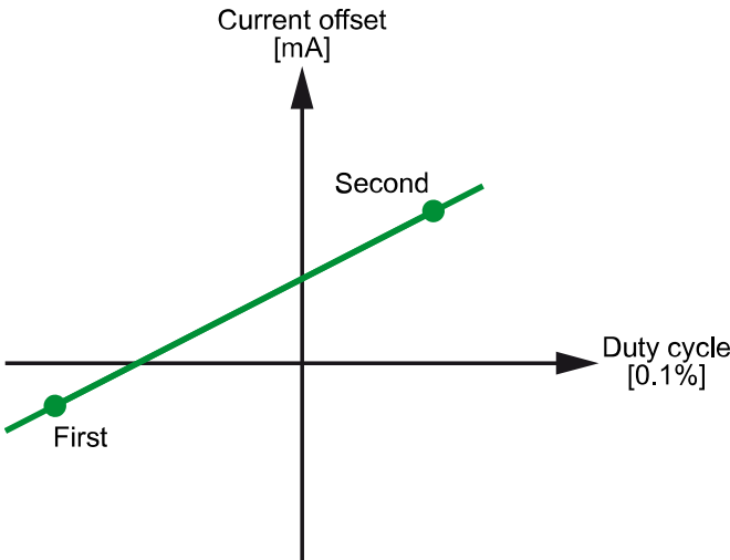
Figure 29. Digital input PWM current set value offset scaling – Set value
