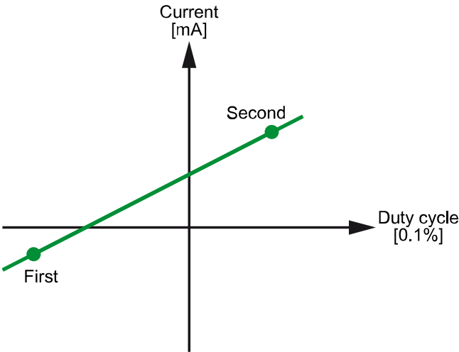
Figure 27. Digital input PWM current set value scaling – Set value
