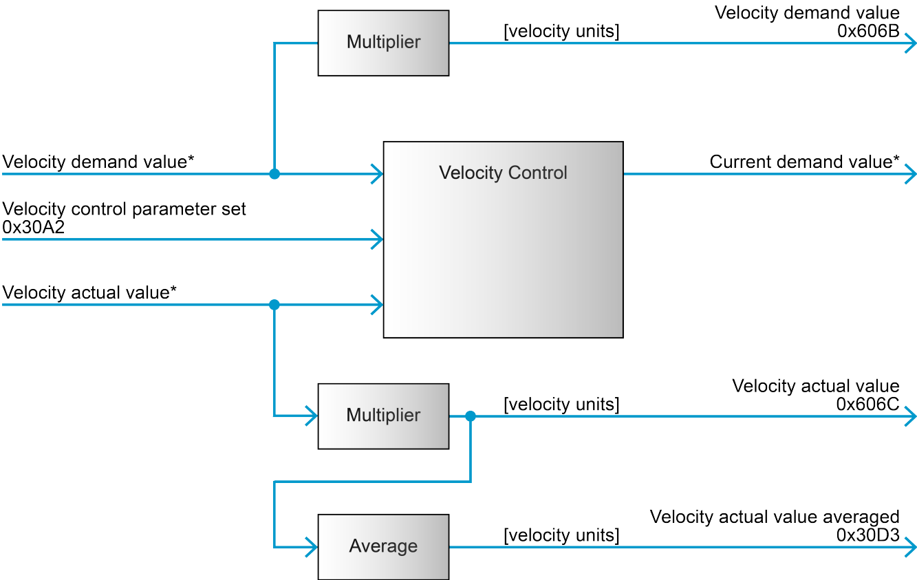
Figure 14. Velocity control function - Block diagram
