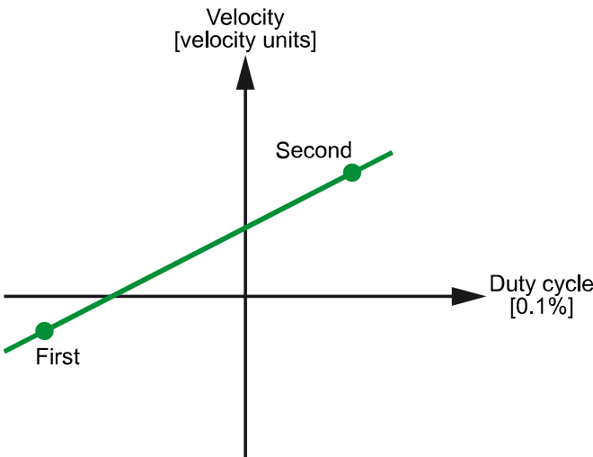
Figure 23. Digital PWM velocity set value scaling – Set value
