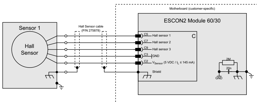
Figure 5-41 Sensor 1 Hall sensor
