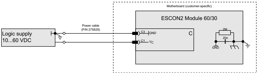
Figure 5-38 Logic supply
