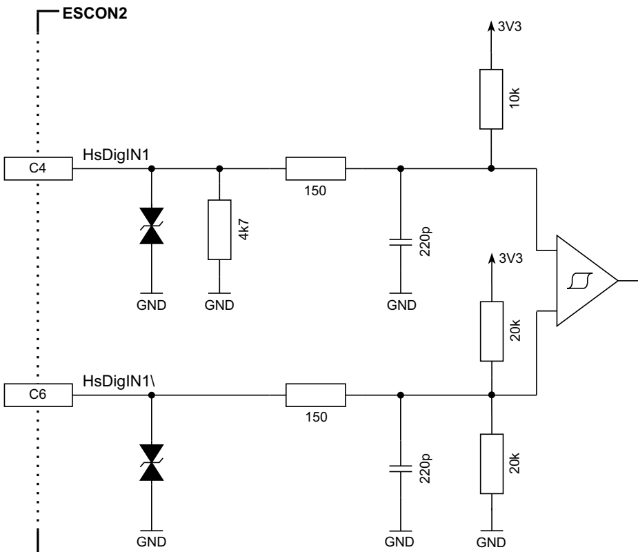
Figure 3-13 HsDigIN1 circuit “differential” (analogously valid for HsDigIN2)
