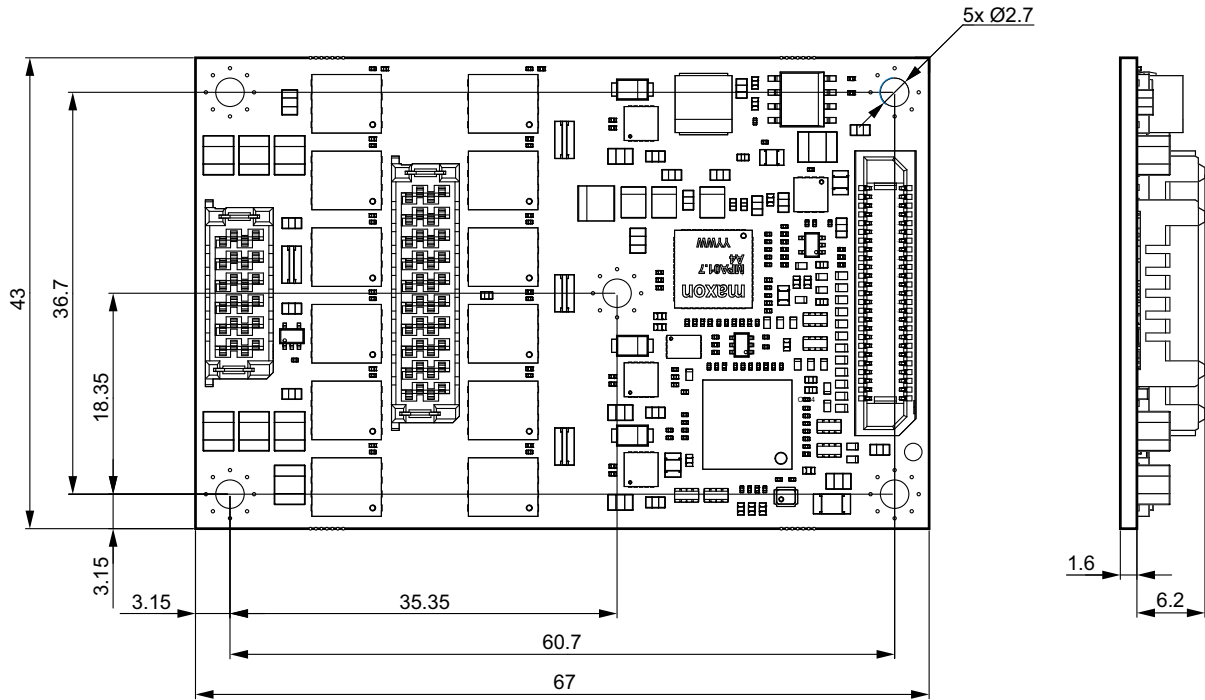
Figure 2-6 Dimensional drawing [mm]
