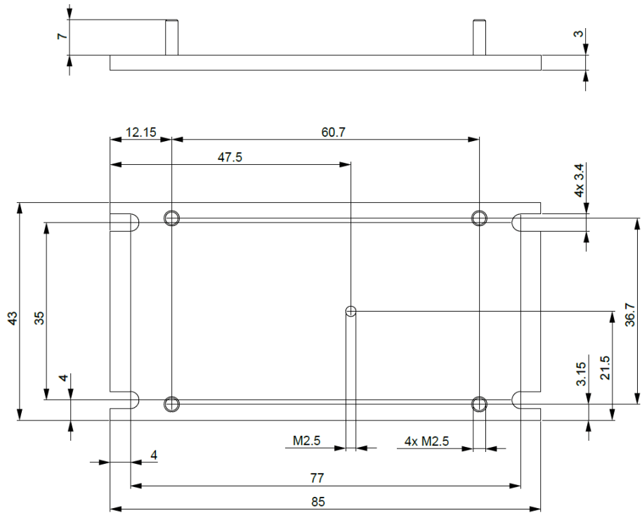
Figure 2-4 Heat spreader dimensional drawing [mm]
