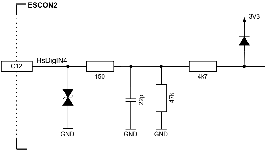
Figure 3-15 HsDigIN4 circuit “single-ended”
