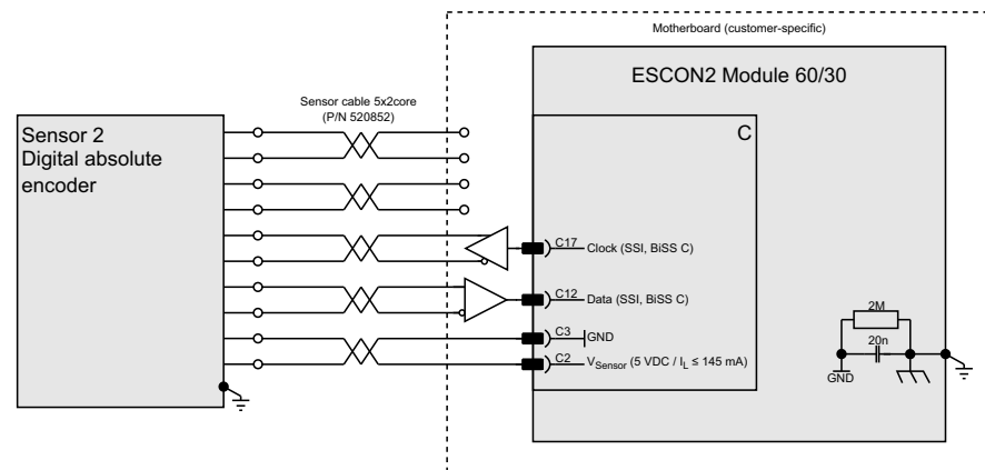
Figure 5-43 SSI / BiSS C unidirectional absolute encoder
