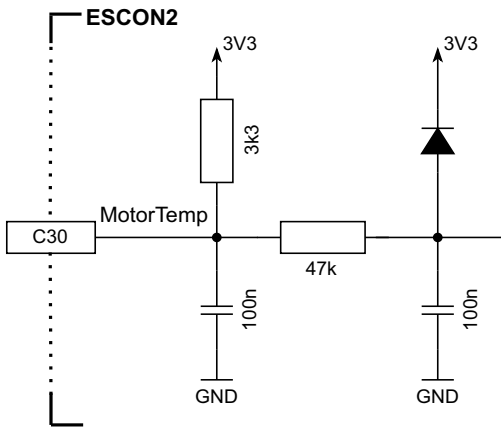
Figure 3-23 Motor temperature circuit
