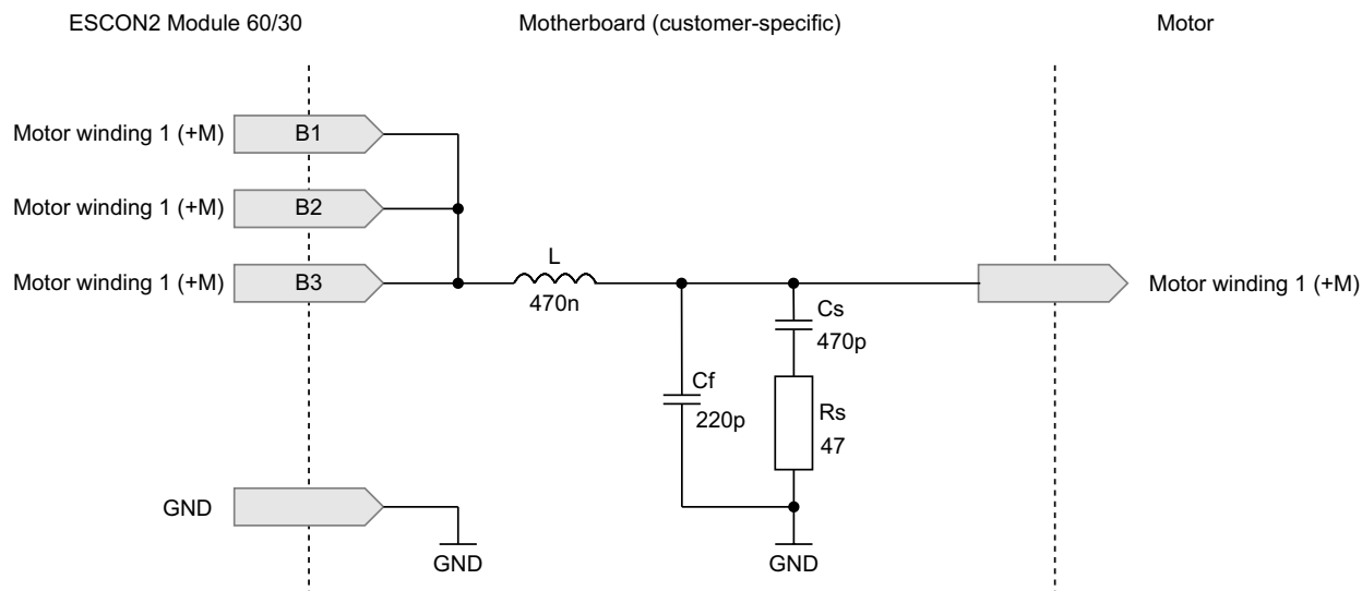
Figure 4-27 Wiring of motor winding 1 (analogously valid for motor winding 2 & 3)
