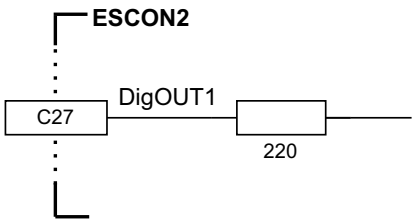
Figure 3-19 DigOUT1 circuit (analogously valid for DigOUT2)
