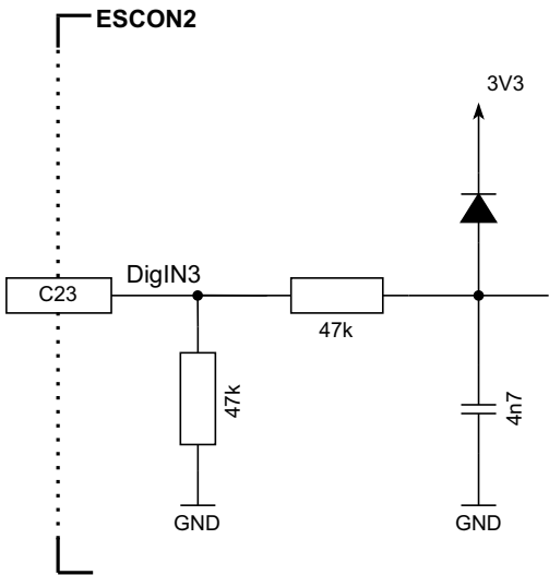
Figure 3-18 DigIN3 circuit (analogously valid for DigIN4)
