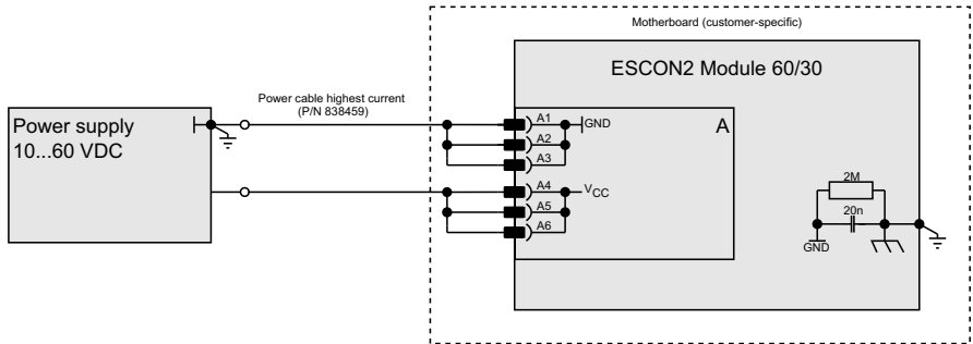
Figure 5-37 Power supply
