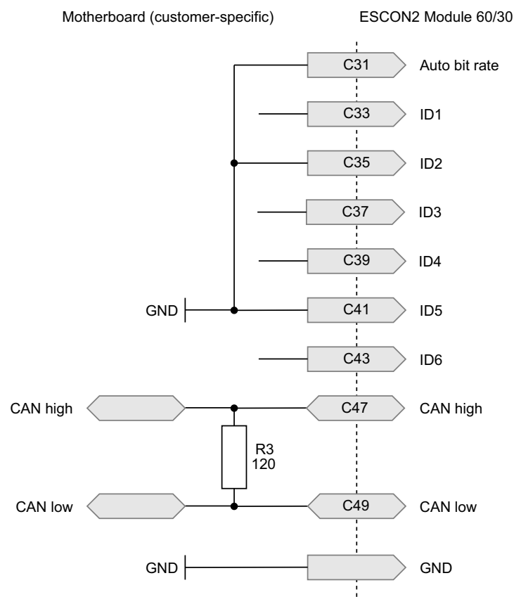
Figure 4-29 Wiring of CAN interface
