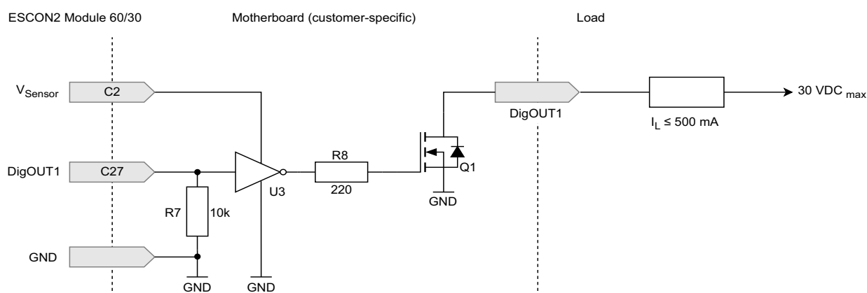
Figure 4-32 Wiring of digital output 1 load switch (analogously valid for digital output 2)
