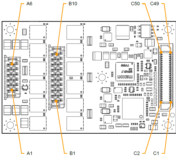
Figure 3-7 Pin assignment
