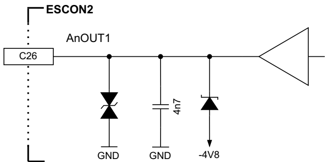
Figure 3-21 AnOUT1 circuit (analogously valid for AnOUT2)
