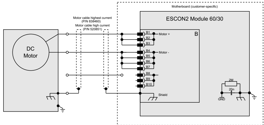
Figure 5-39 DC motor
